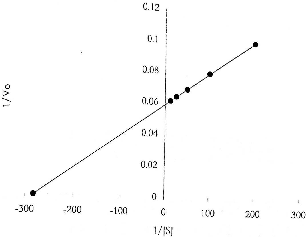
Fig- 28: Linweaver-Burk double reciprocal plot for the determination of K_m value of the purified betel leaf polyphenol oxidase.
