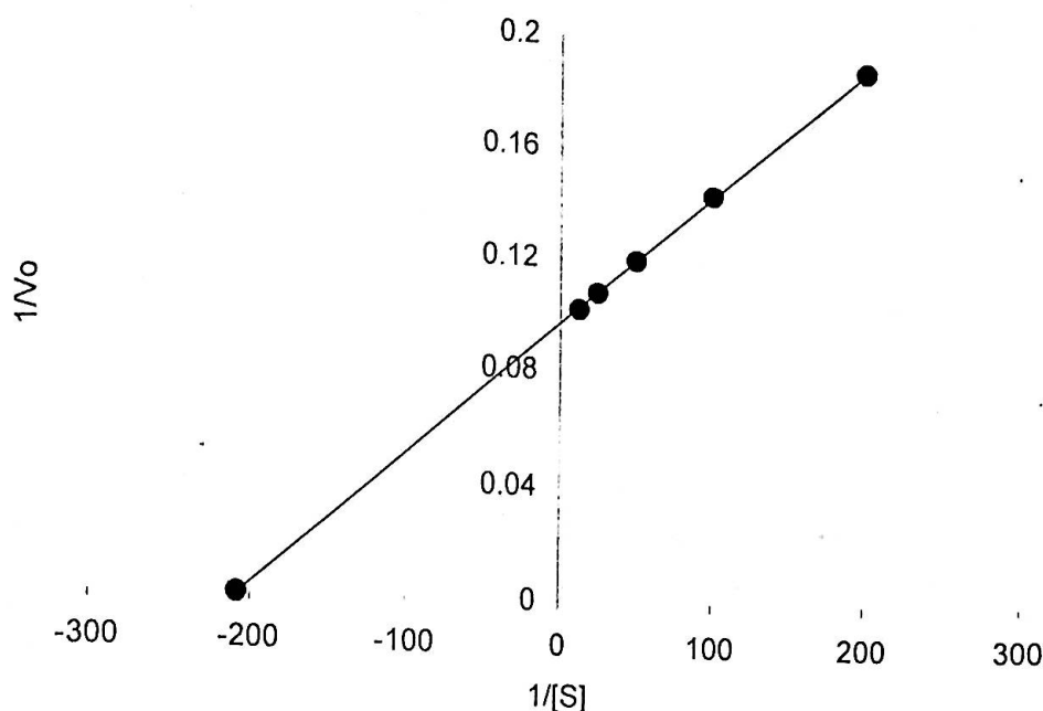
Fig- 25: Lineweaver-Burk double reciprocal plot for the determination of K_m value of the purified betel leaf AIV II.
