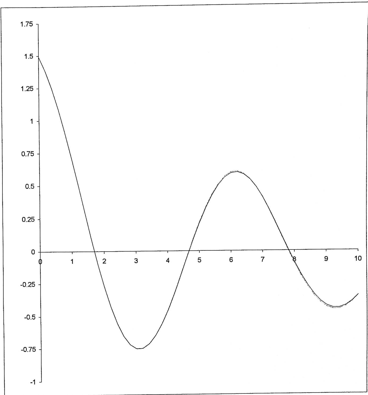
Fig. 2.2 Solution of equation (2.1) obtained by perturbation theory (solid line) in which a , b and c are evaluated by (2.21), and numerical integration (dotted line) for \lambda=0.8 , \omega=1.0 , \varepsilon=-0.1 and f=-2(x+\lambda x)+x^3 with the initial conditions a_0=0.5 , b_0=1.0 and c_0=0 or, [x(0)=1.49203, \dot{x}(0)=-0.49000, \ddot{x}(0)=-0.58204] .
