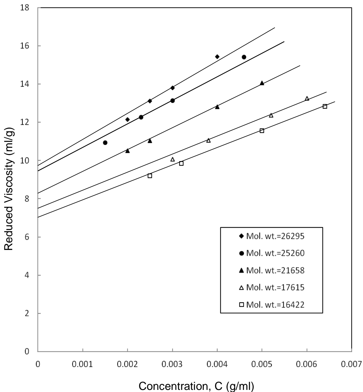
Fig. 3.2 : Plots of concentration Vs reduced viscosity for maleic acid-butane-1,4-diol polyester of different fractions in ethylacetate at 26°C.
