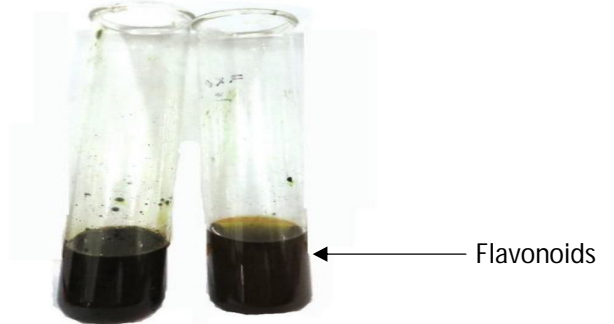
Fig. 87: Flavonoids
