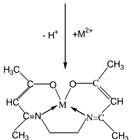
Bis(acetylacetonone)ethylenediamine
