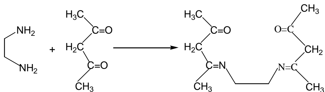
Bis(acetylacetonone)ethylenediamine
