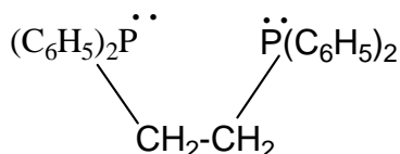
Bisdiphenylphosphinoethane
