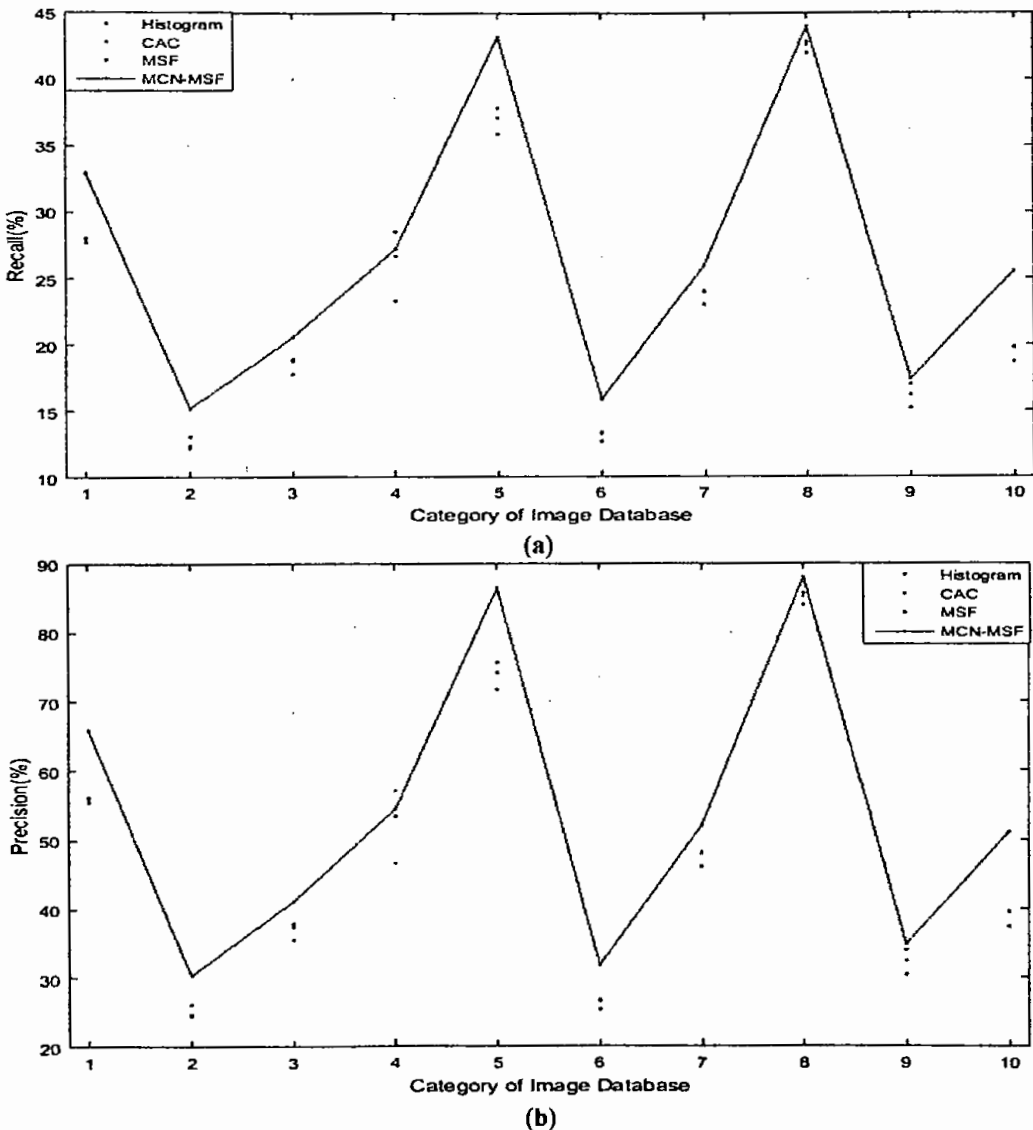
Fig. 4.5 Category-wise (inWANG1000db) performance at n=50, in terms of a) Recall and b) Precision for Histogram, CAC, MSF and MCN-MSF.
