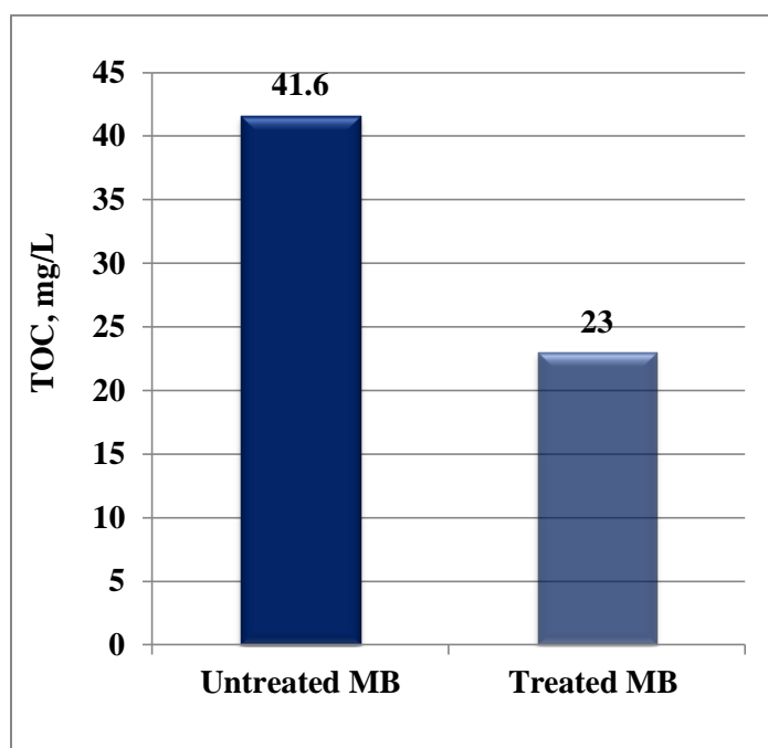
Figure 4.12 Mineralization of 40 ppm MB by photocatalytic treatment (Catalyst = ZnO, Catalyst conc. = 200 ppm, pH= 4, Reaction time = 3 hrs, H 2 O 2 = 600 ppm)
